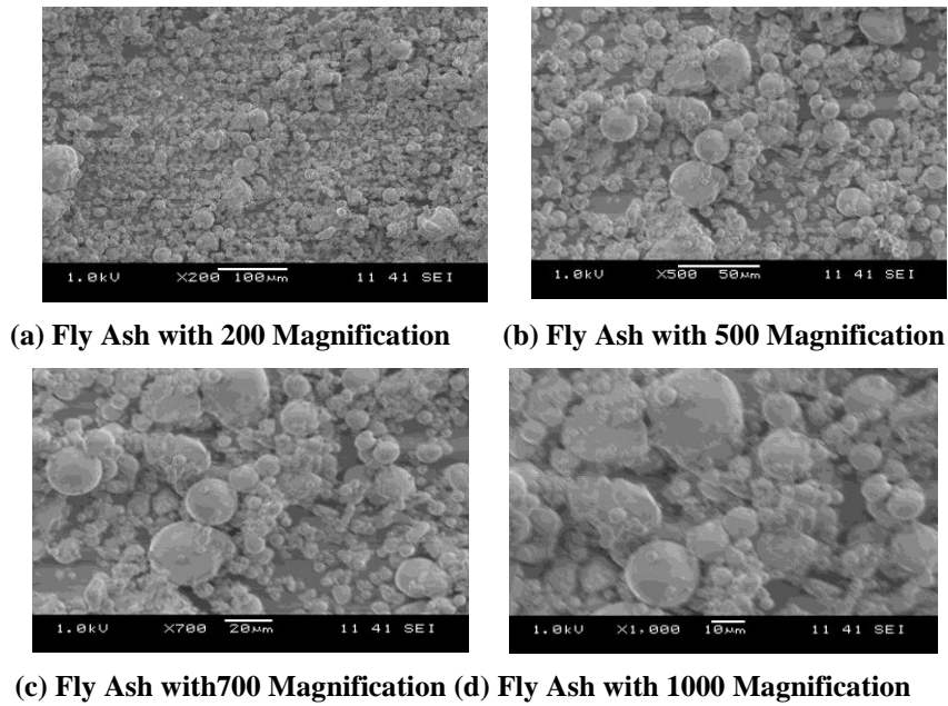
Figure 1: SEM Images of Fly Ash
